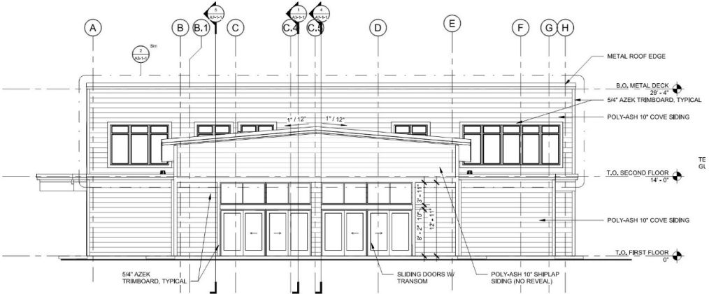
3 NORTH ELEVATION 1/8" = 1'-0"
