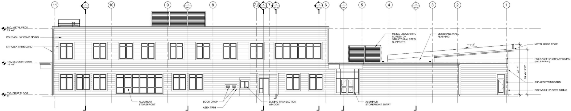
1 EAST ELEVATION 1/8" = 1'-0"
